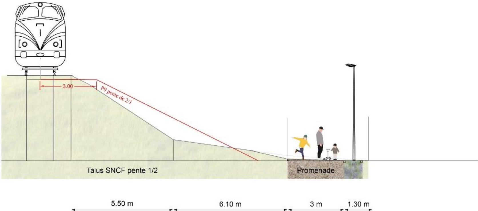
COUPE C3
